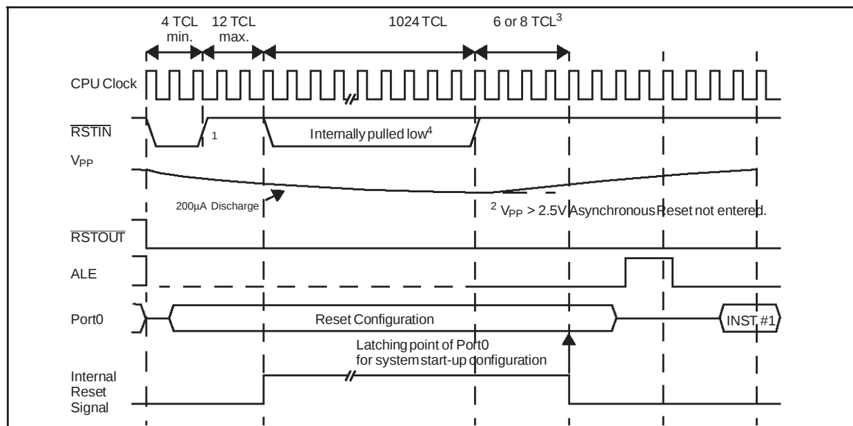
Figure 10 : Synchronous Warm Reset: Short low pulse on \overline{\text{RSTIN}}
