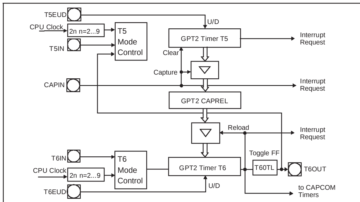
Figure 7 : Block Diagram of GPT2
